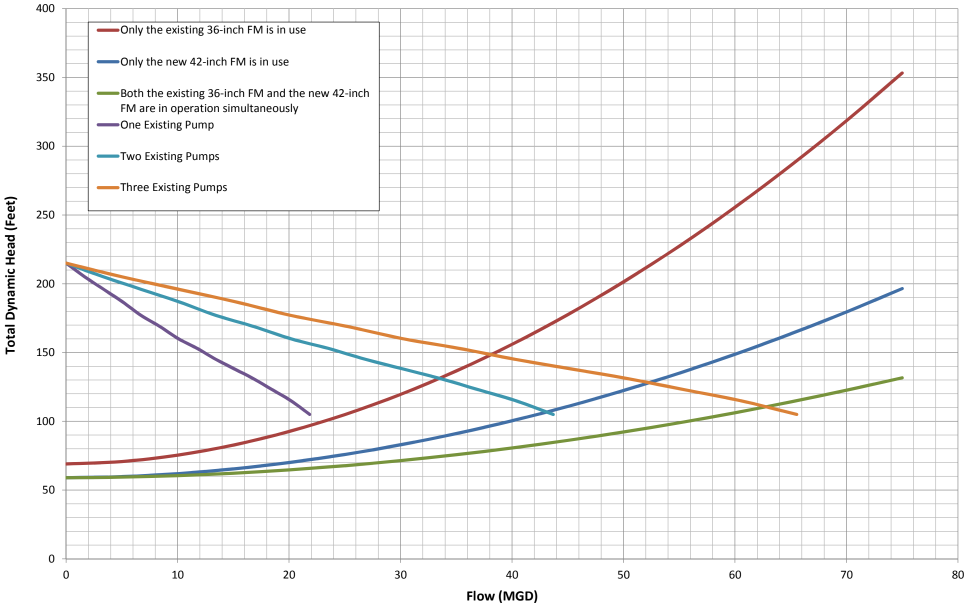
Brandon Road Pump Station Total Dynamic Head Curves with Existing Pump Curves
